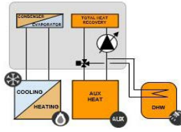
HYGR1V+VACSR (2 - pipes)
